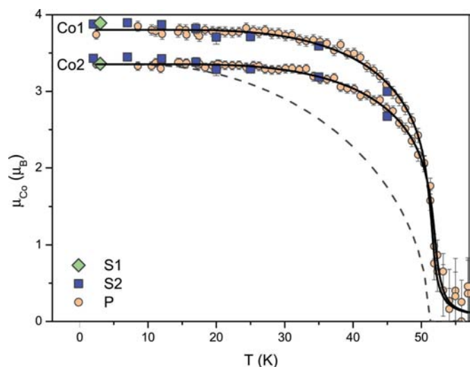
Figure 8 Temperature dependence of the Co magnetic moment for \text{Co}_2\text{SiO}_4 . The experimental data from the single-crystal (S1,S2) and powder (P) neutron diffraction measurements are shown together with the fitting curves (solid lines) in a modified molecular-field model [equation (6)]. Error bars are smaller than the symbols if not given. The dashed line is shown to illustrate the deviation of \mu_{\text{Co}2}(T) from the conventional molecular-field model [equation (4)].
