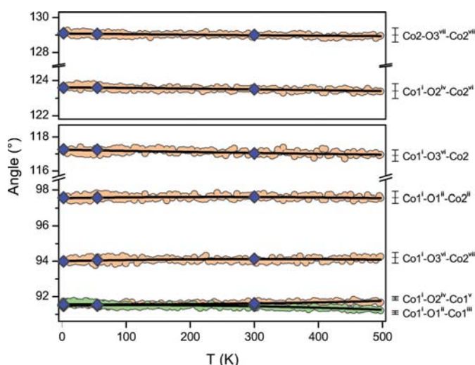
Figure 7 Temperature dependence of the Co–O–Co angles for \text{Co}_2\text{SiO}_4 . Circles mark the results of the powder neutron diffraction measurements (error bars shown at the right), whereas rhombs mark the results of the single-crystal neutron diffraction measurements (error bars from the refinement are smaller than the symbols). The fits are used as guides to the eye. See Table 6 for the symmetry codes.
