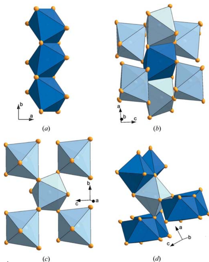
Figure 2 All possible arrangements of the \text{CoO}_6 octahedra in \text{Co}_2\text{SiO}_4 (see text for details). (a) \text{Co1O}_6 neighbours of \text{Co1O}_6 , (b) \text{Co2O}_6 neighbours of \text{Co1O}_6 , (c) \text{Co2O}_6 neighbours of \text{Co2O}_6 and (d) \text{Co1O}_6 neighbours of \text{Co2O}_6 .
