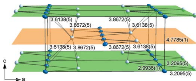
Figure 1 Perspective drawing of the arrangement of the \text{Co}^{2+} ions in layers perpendicular to the c axis (space group Pnma ) of \text{Co}_2\text{SiO}_4 . Some Co–Co distances are marked for clarity.
