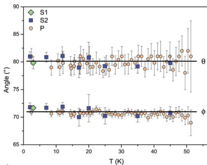
Figure 9 Temperature dependencies of the angles which describe the direction of the Co1 magnetic moment for \text{Co}_2\text{SiO}_4 . The experimental data from the single-crystal (S1,S2) and powder (P) neutron diffraction measurements are shown. Error bars are smaller than the symbols if not given. The solid lines represent a linear fit.
